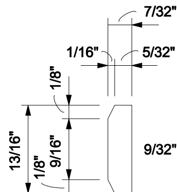
REAR SCREW POST
