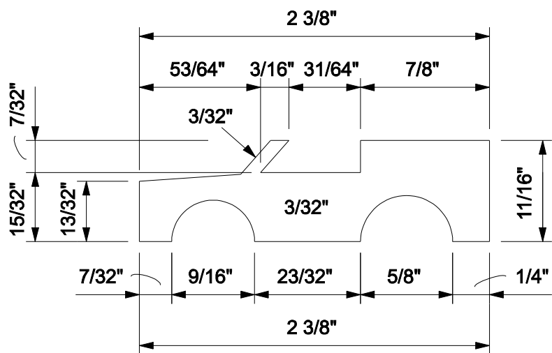
DRIVER SIDE AND PASSENGER SIDE PANELS
