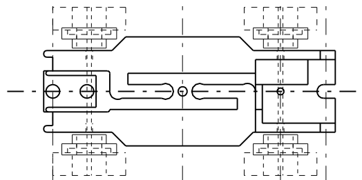
UNDERSIDE VIEW
